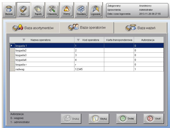
Database window
