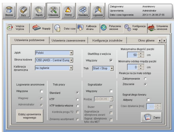
Configuration panel
